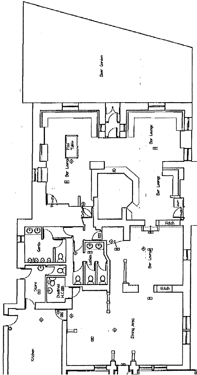
Ground Floor Plan LDA=425m 2
